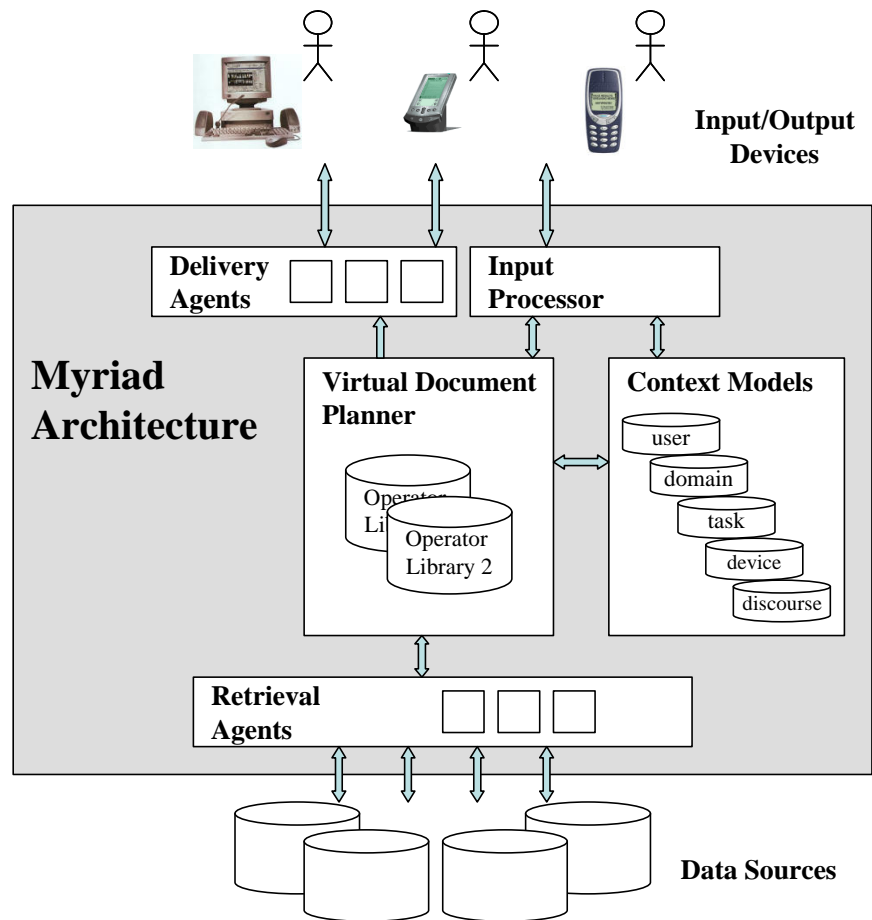
Fig. 1. The Myriad Architecture
