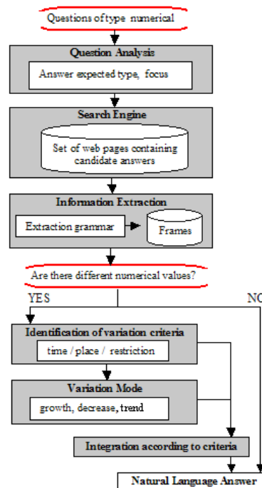
Figure 1: Architecture
